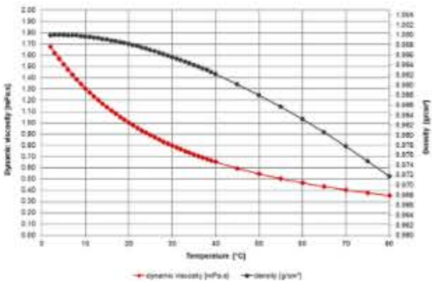
Water - dynamic viscosity and density over temperature
